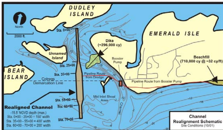
BOGUE INLET CHANNEL / WESTERN PHASE BEACH NOURISHMENT PROJECT
